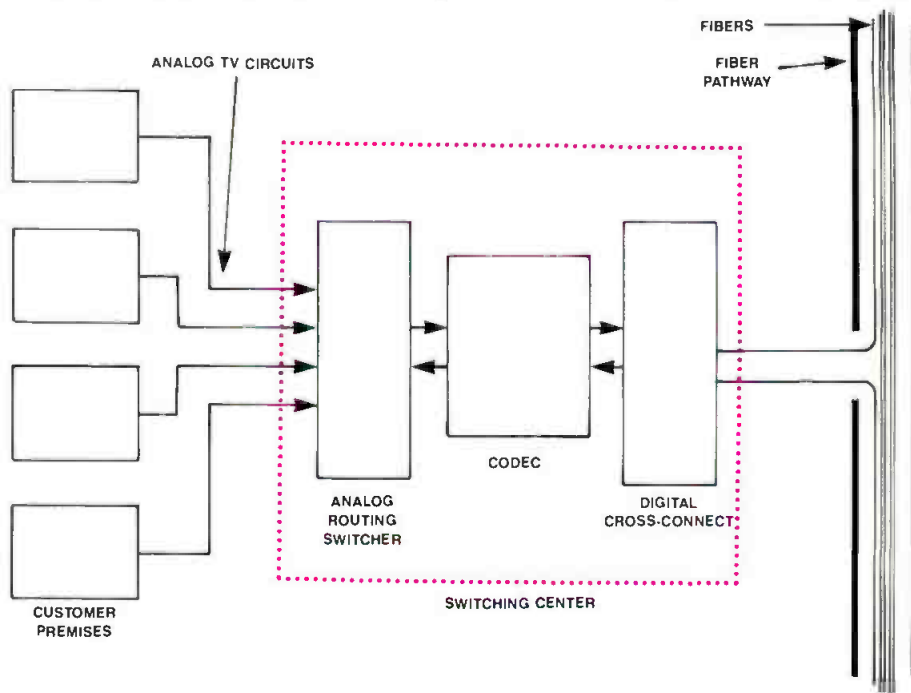
Figure 3. One national fiber optic uses DS-3 channels to transport TV audio and video around the country. At various cities, fibers are pulled from the pathway, run into a cross-connect and fed to an analog switch for distribution.
